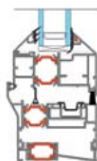
Sill Detail
